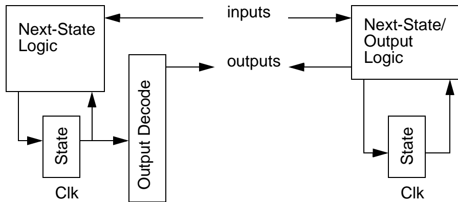
Figure 2. Moore and Mealy Machines
